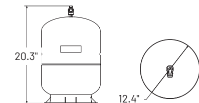
5-gallon hydropneumatic tank
